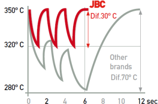
B/ PROCESS FOR 3 SOLDER JOINTS
