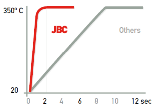
A/ TIME TO REACH 350° C
